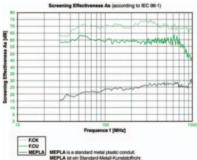
Schirmcharakteristiken / screening characteristics:
