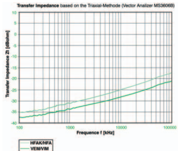
Transferimpedanz / Transfer impedance:
